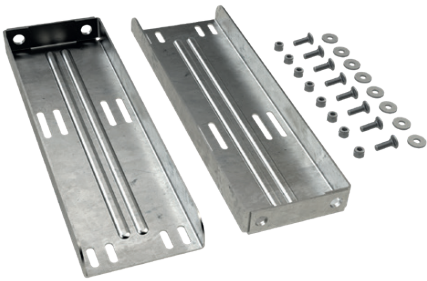
88472 Hot galvanized steel brackets with Geomet coated fixing kit.
