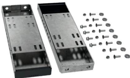
88712 Hot galvanized steel brackets with Geomet coated fixing kit.
